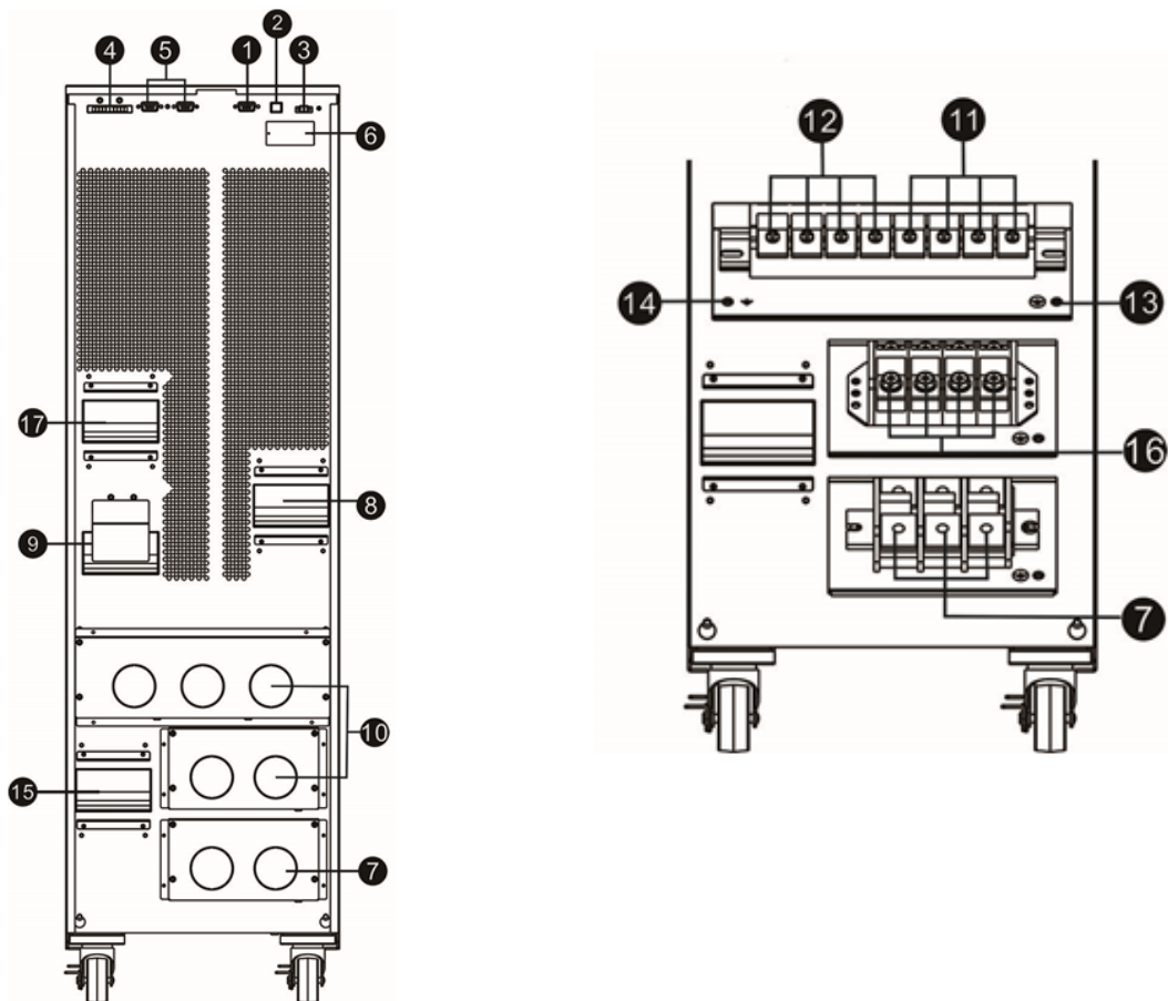
Diagram 1: Rear panel
