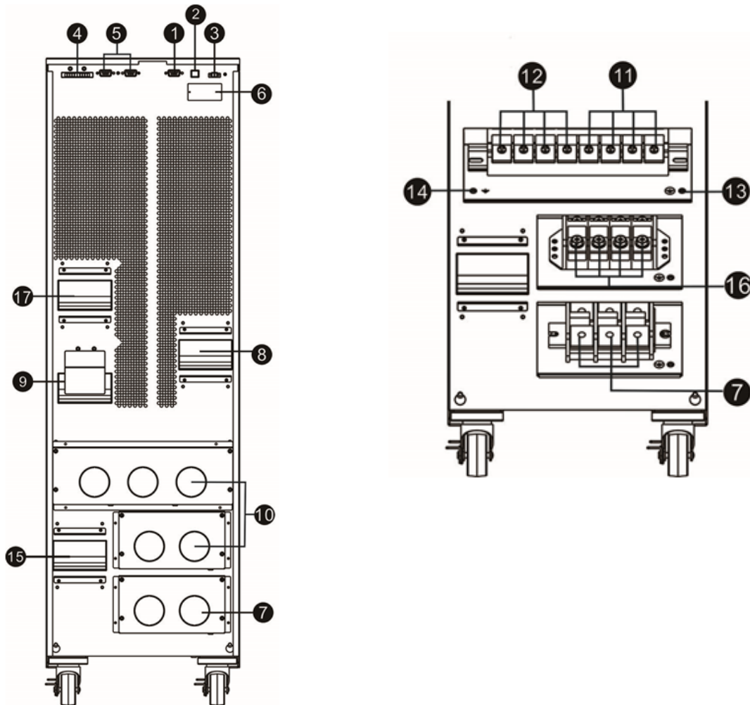
Diagram 1: Rear panel
