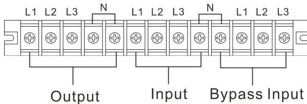
33 Schematic diagram of the connection of short circuit sheet copper
